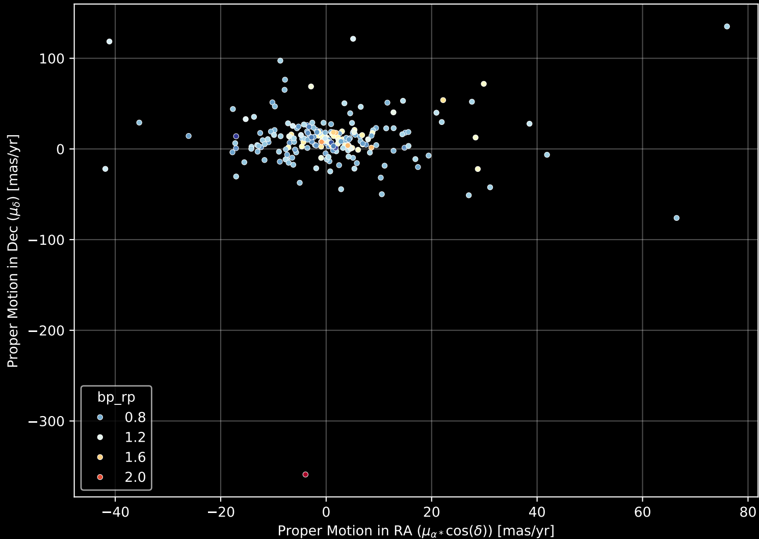
GALAH DR4 Field: [7238] Proper Motion Diagram (n= 209)
