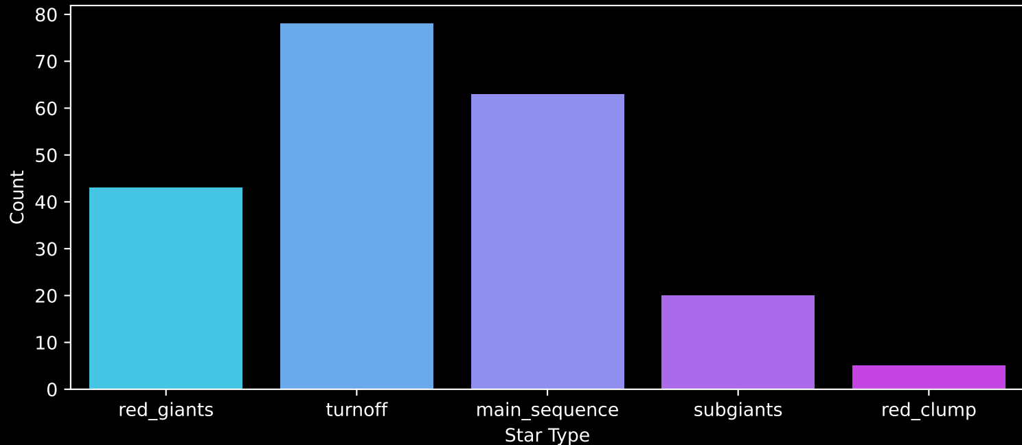
GALAH DR4 Field: [7238] Count plot of Star Type
