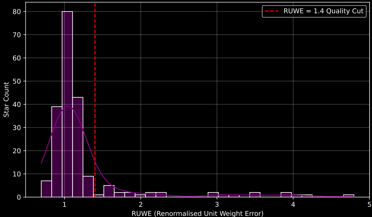
GALAH DR4 Field [7238] RUWE Distribution (n= 204)
