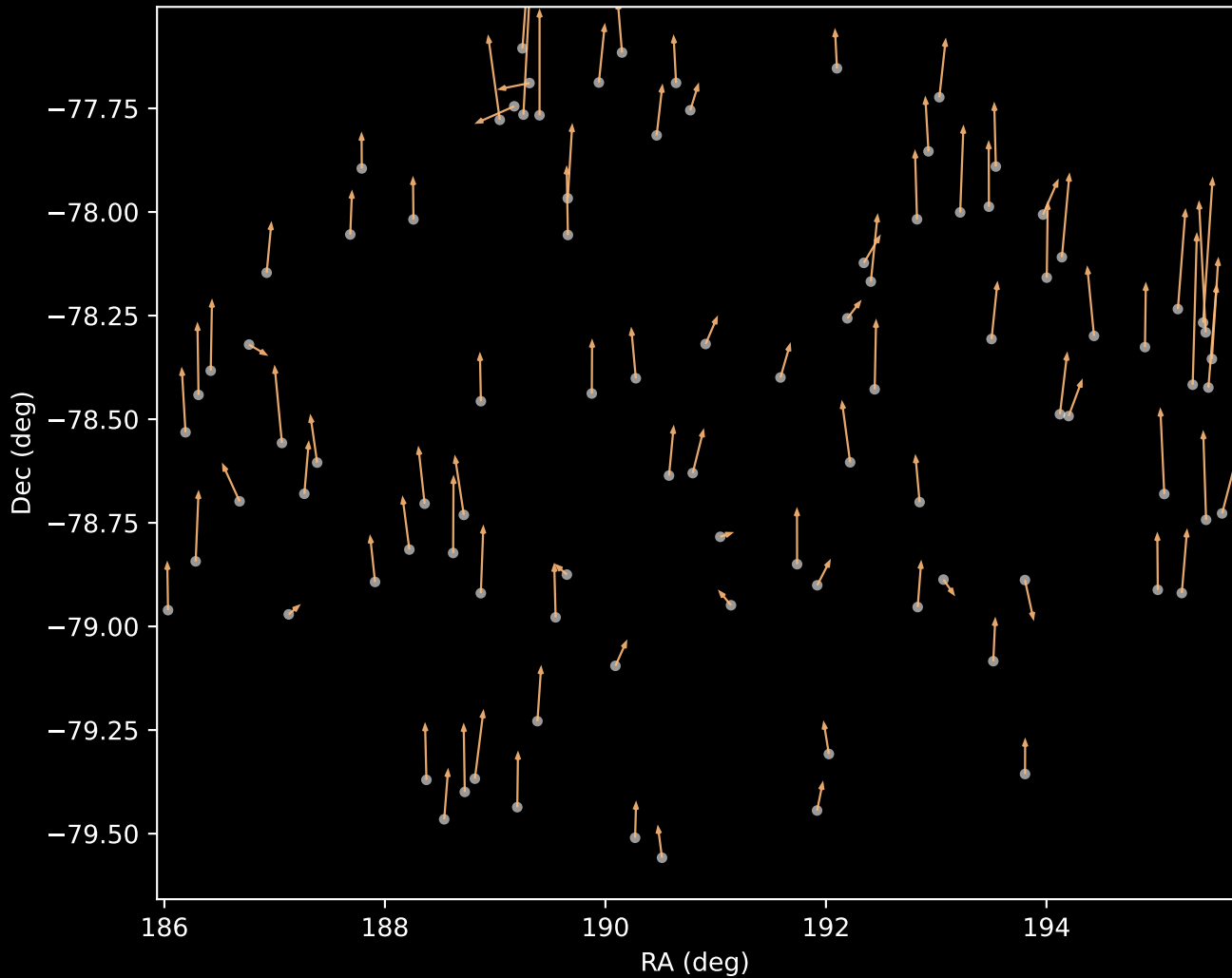
GALAH DR4 Cluster 3 Proper Motion Vectors (n=95)
